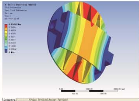
Finite element structural analysis
